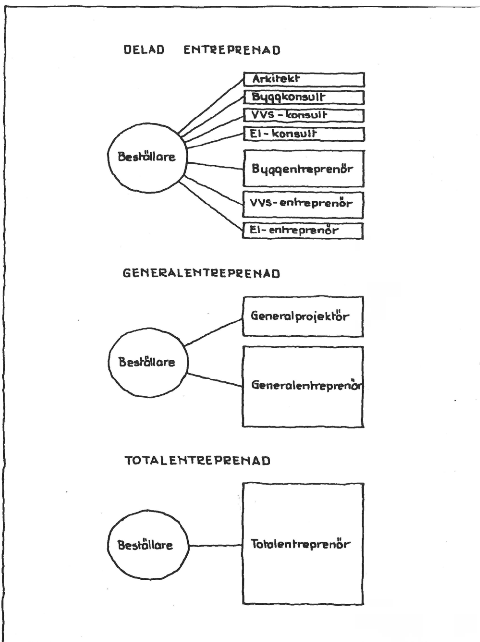
Fig. 1:6 Entreprenadformer, principalschema.
